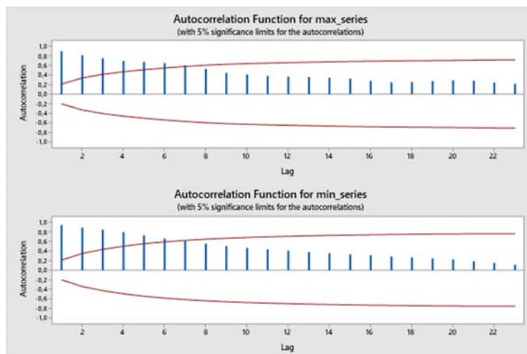
Figure 4 – Autocorrelation functions
