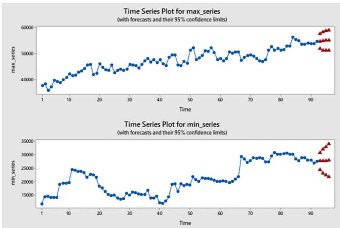
Figure 12 – Predicted values
